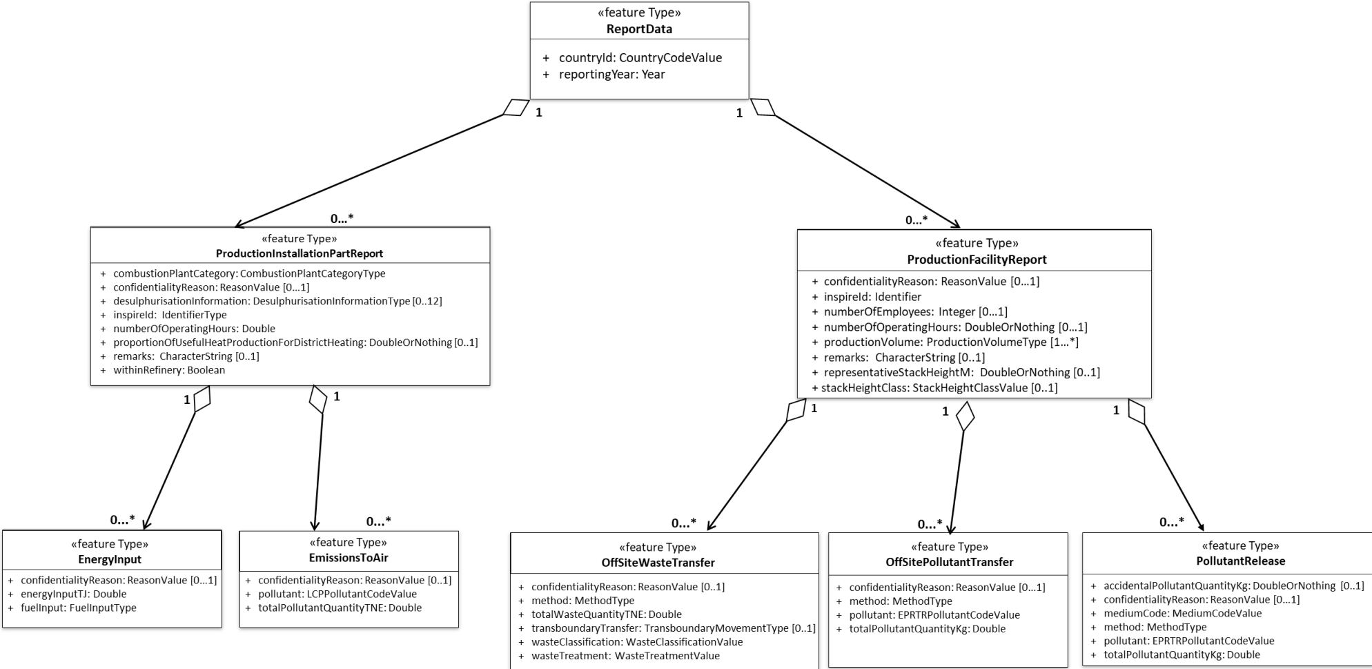
Figure 3 Diagram of the E-PRTR+LCP dataflow feature types
