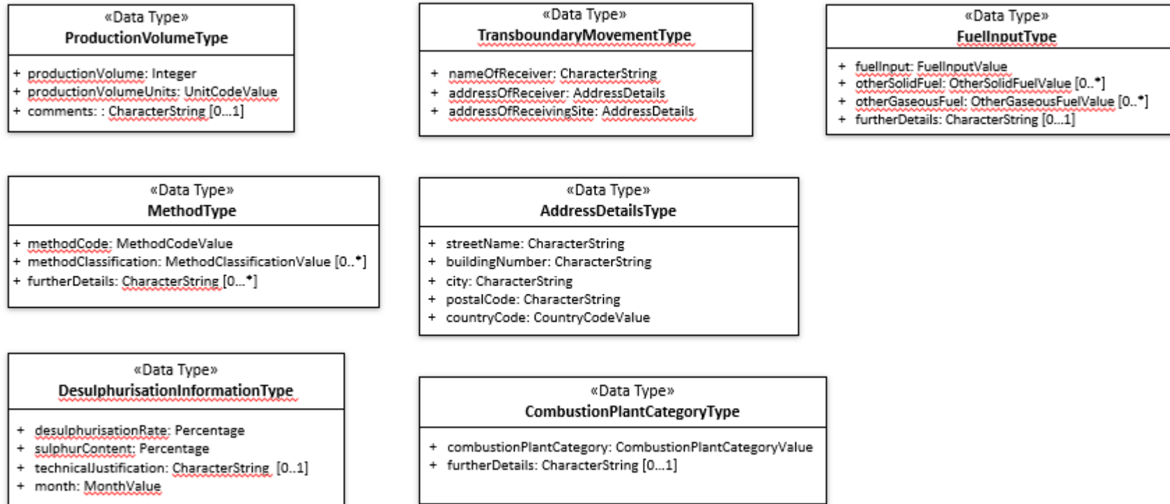
Figure 4 Diagram of the E-PRTR+LCP dataflow data types
